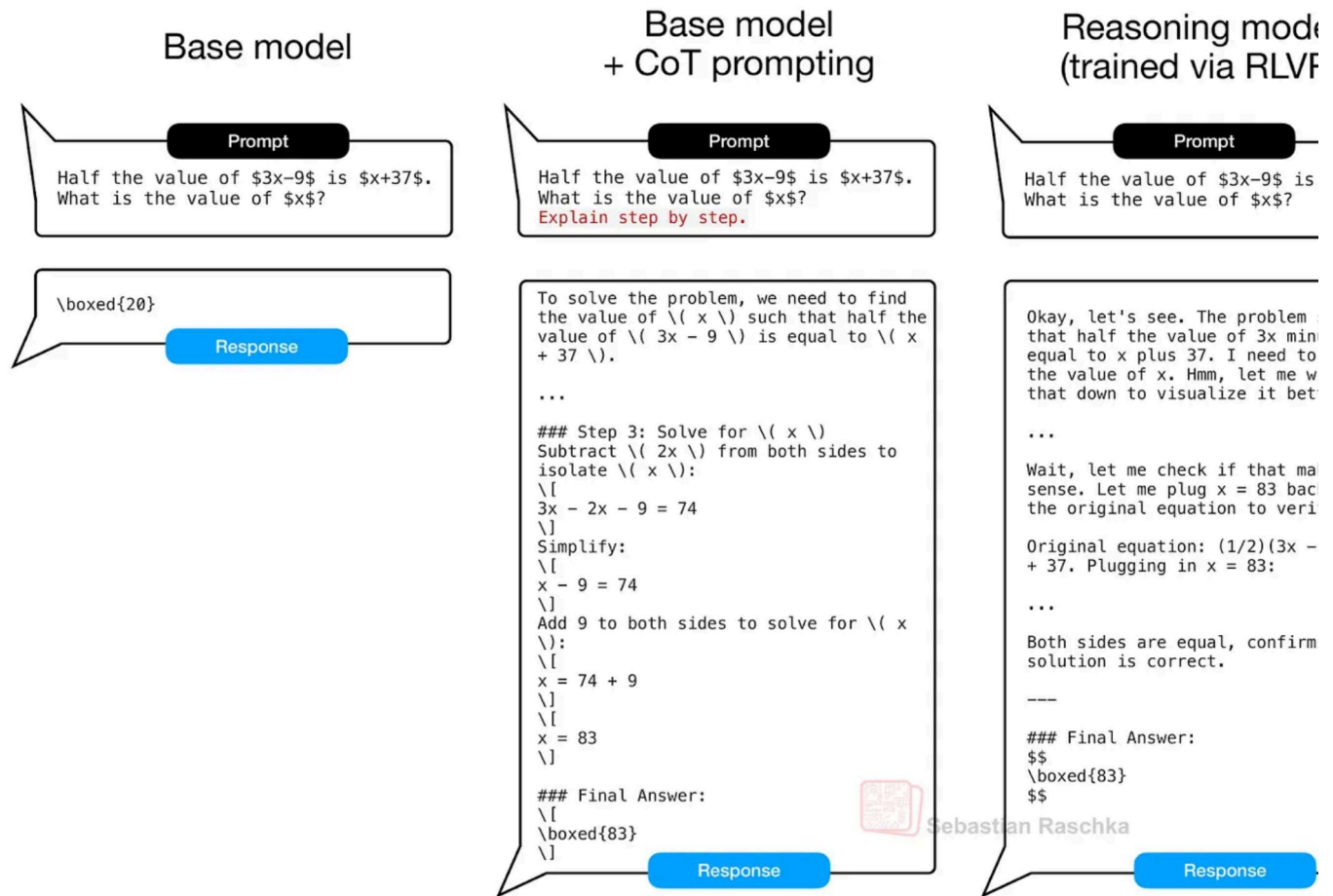
Figure 4: Real outputs via Qwen3 0.6B base and reasoning model on a MATH-500 test set query. When using CoT prompting, the base model explains the answer more often (center), similar to the reasoning model, which can improve the answer accuracy.
