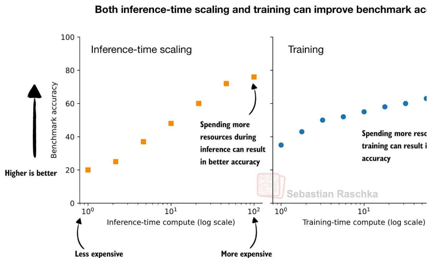
Figure 1: Spending additional resources during inference (left) and training (right) generally improves the model's accuracy.
