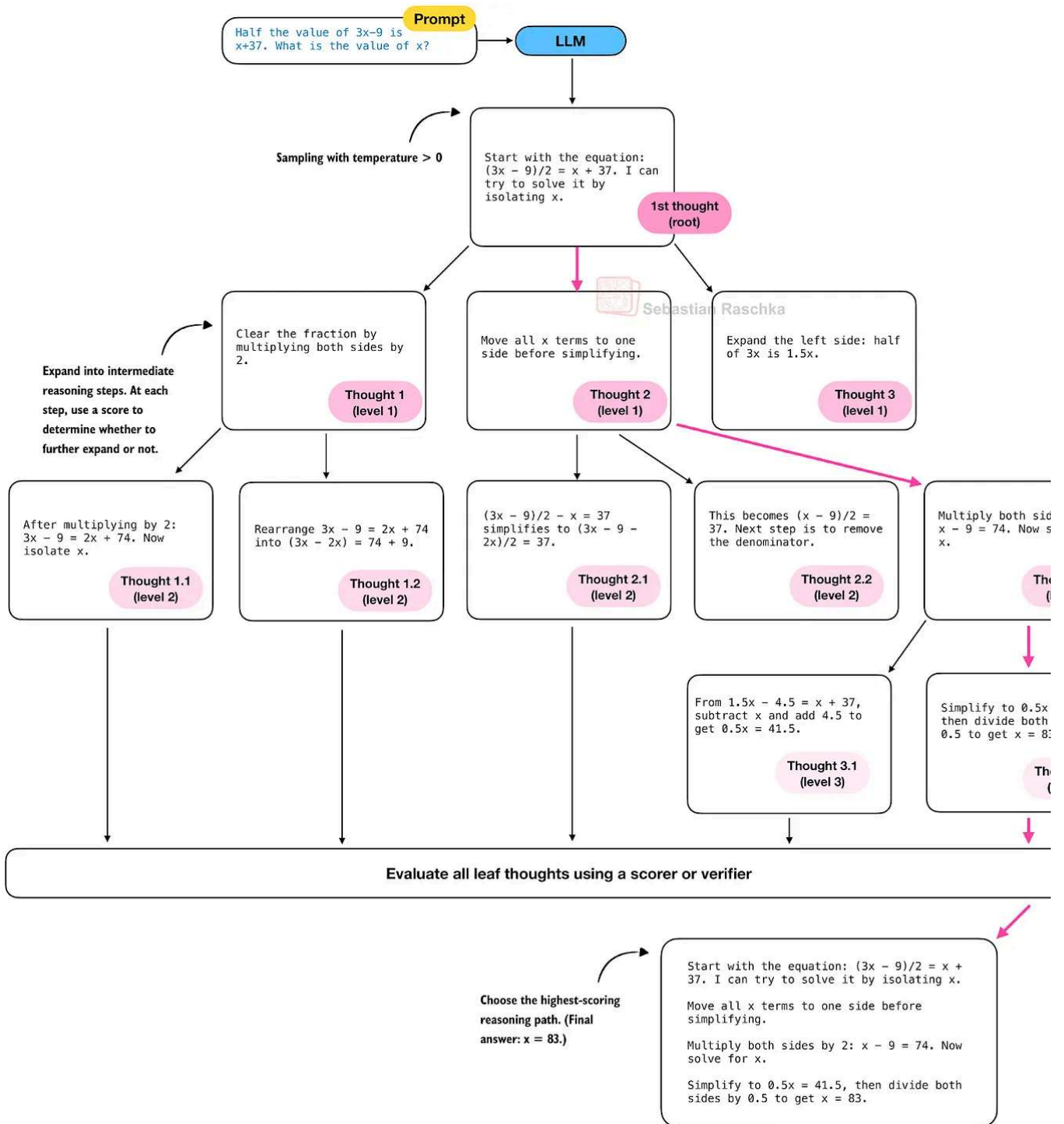
Figure 11: An illustration of Tree-of-Thoughts sampling.
